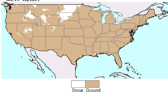
Snow Cover (USAF 557th WW) Oct. 14 - 20, 2019
